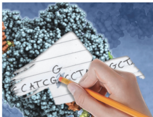
Base Editors
